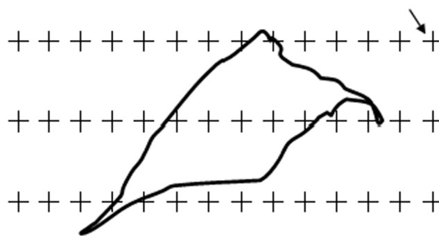
Fig.1. Schematic drawing of a photomicrograph superimposed by the test point system.
