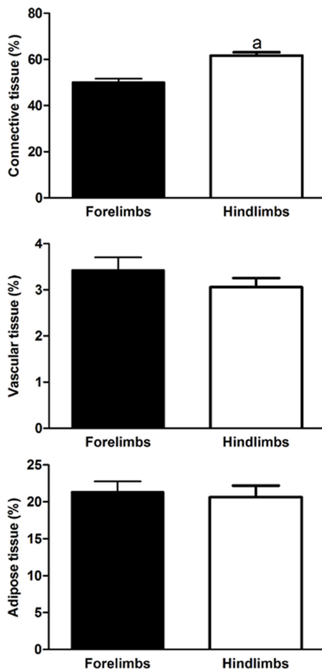
Fig.4. Mean and standard errors ( n=12 ) of connective, adipose and vascular tissue in bovine digital cushions. Letter 'a' on the column indicates significant difference ( p \leq 0.05 ).
